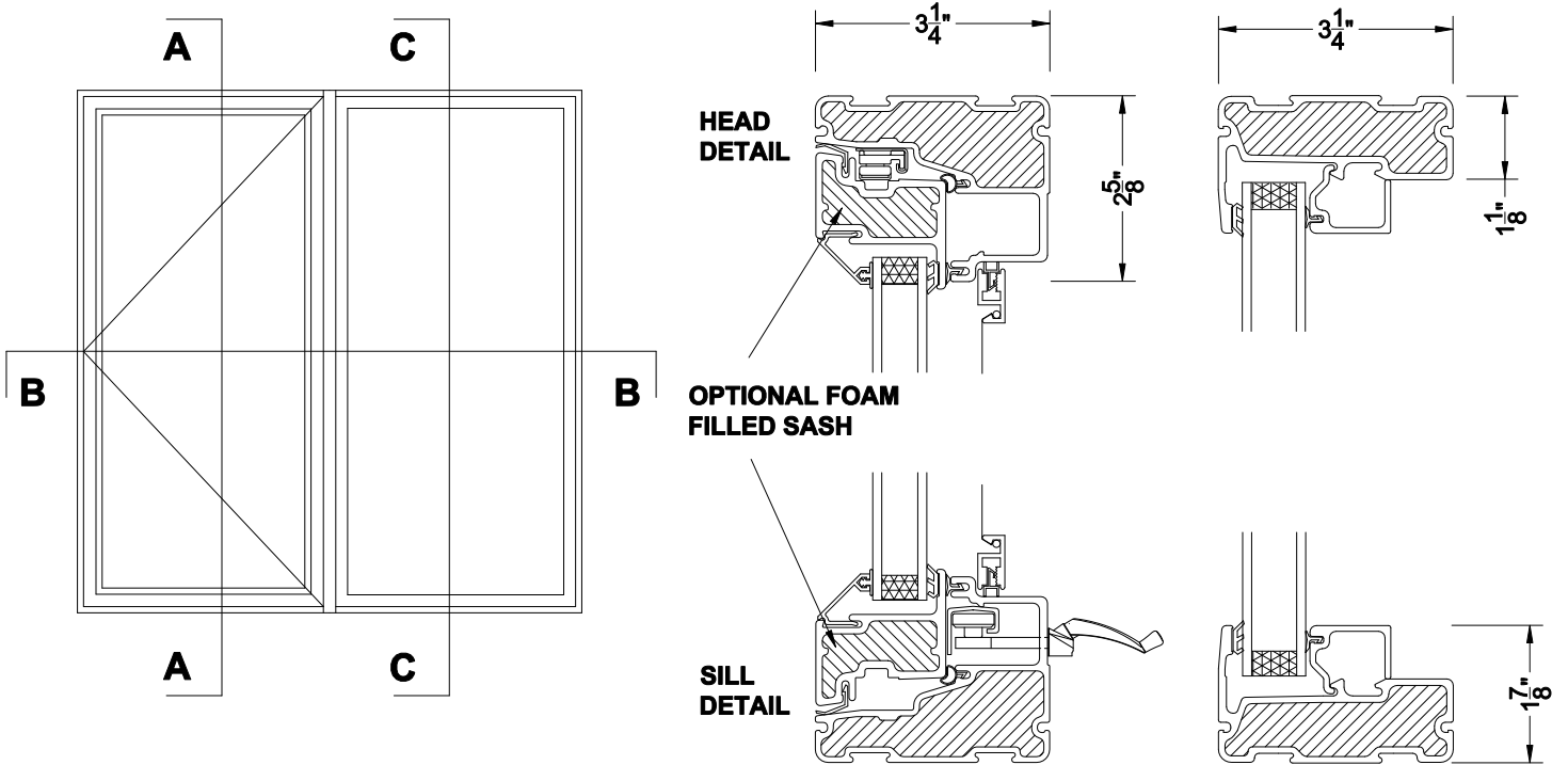
CASEMENT / FIX Exterior View closed back frame casment
