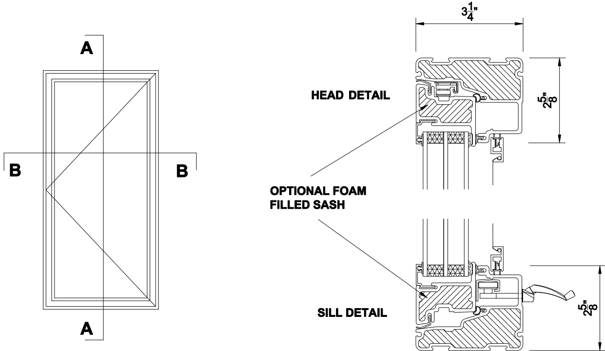
CASEMENT WINDOW EXTERIOR VIEW CLOSED BACK FRAME
