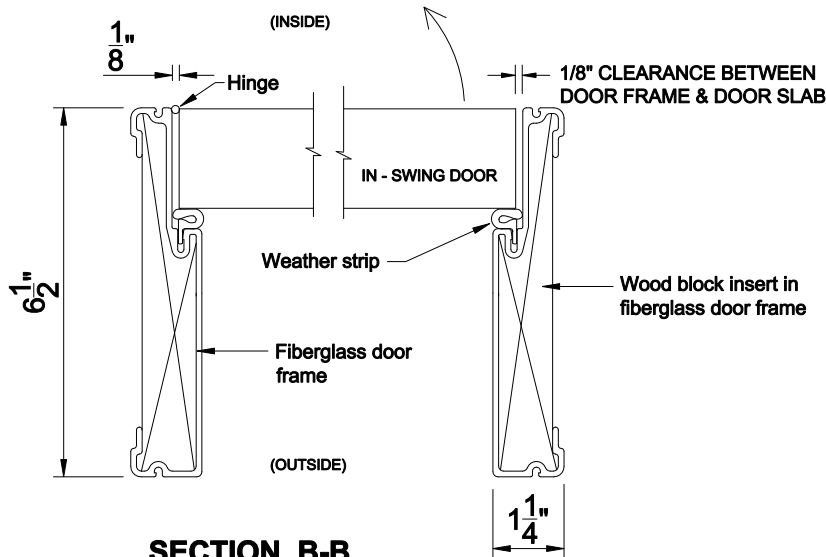
SECTION B-B
