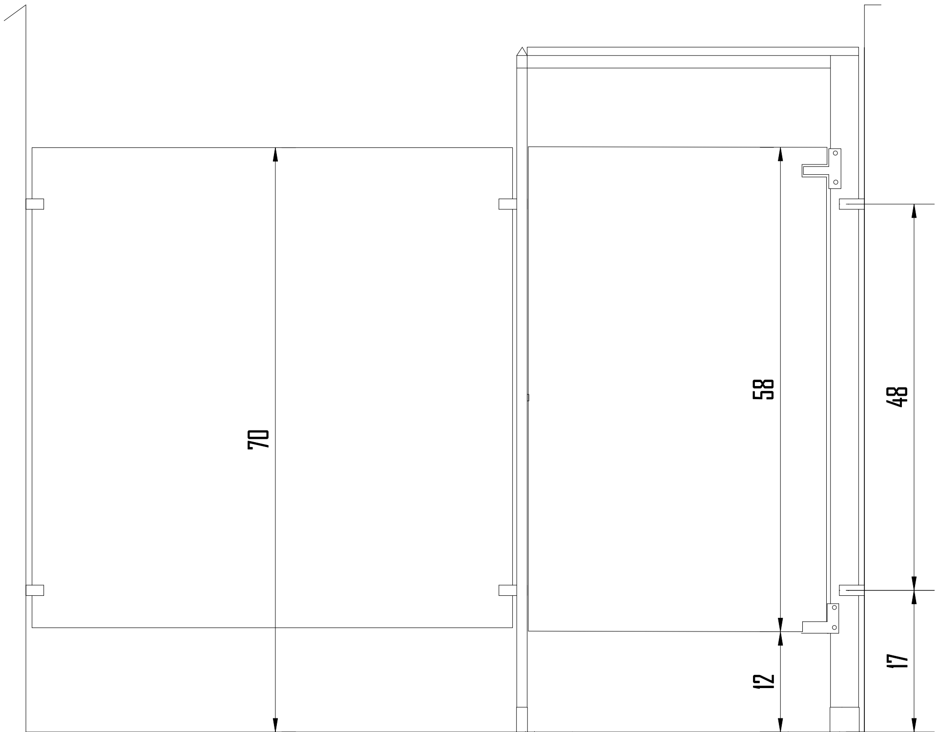
FRONT VIEW ELEVATION USING FLAT STRIKE CONDITION
