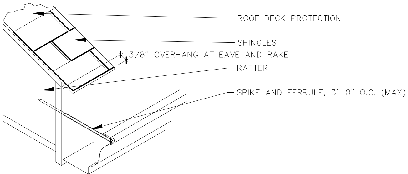
○ HANGING GUTTER INSTALLATIONS — SLOPED ROOF GAF RESIDENTIAL ROOFING SHINGLES
