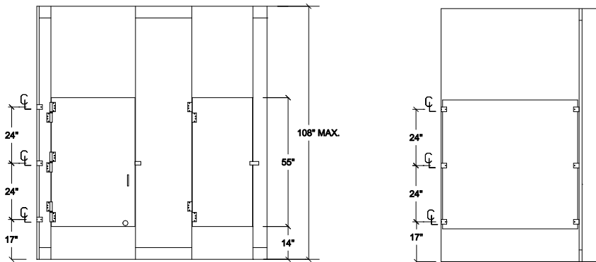
A TYPICAL FLOOR TO CEILING ELEVATION
