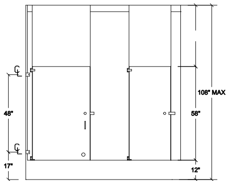
A TYPICAL CEILING HUNG ELEVATION
