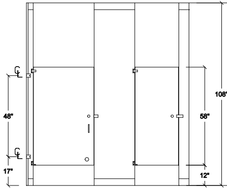
A TYPICAL FLOOR TO CEILING ELEVATION
