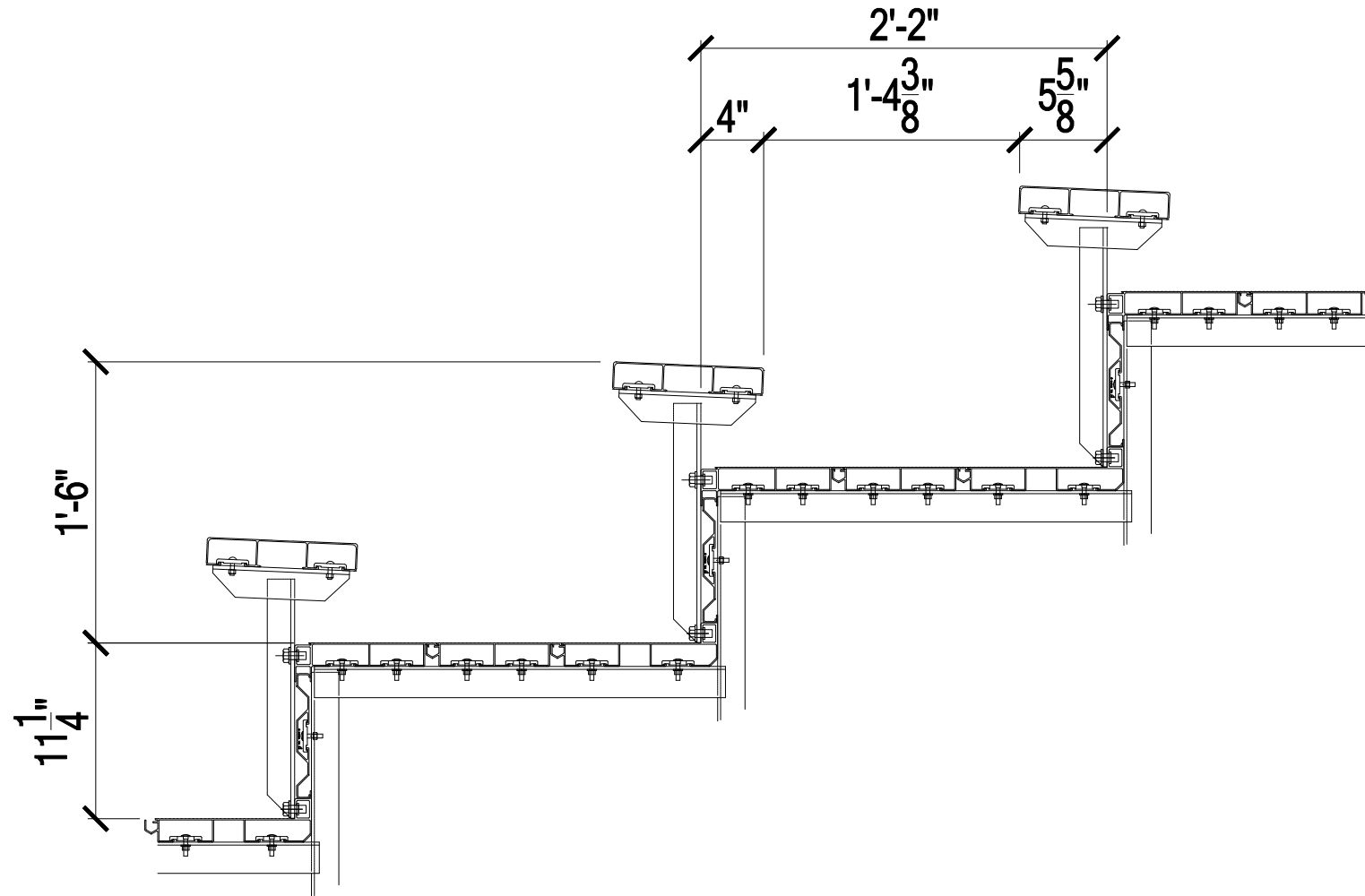
ALUMINUM PLANKING - INTERLOCKING DECK (11 1/4" RISE / 26" TREAD)
