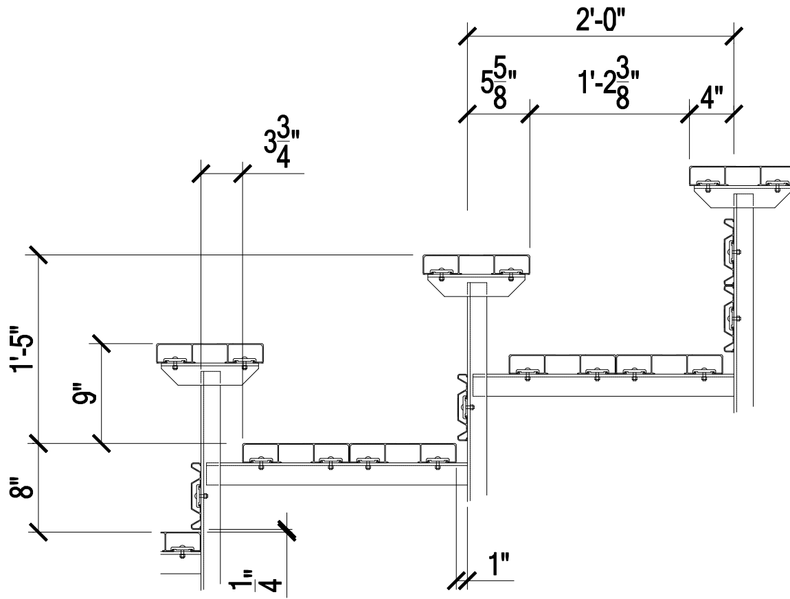
ALUMINUM PLANKING – SEMI-CLOSED DECK (8" RISE / 24" TREAD)
