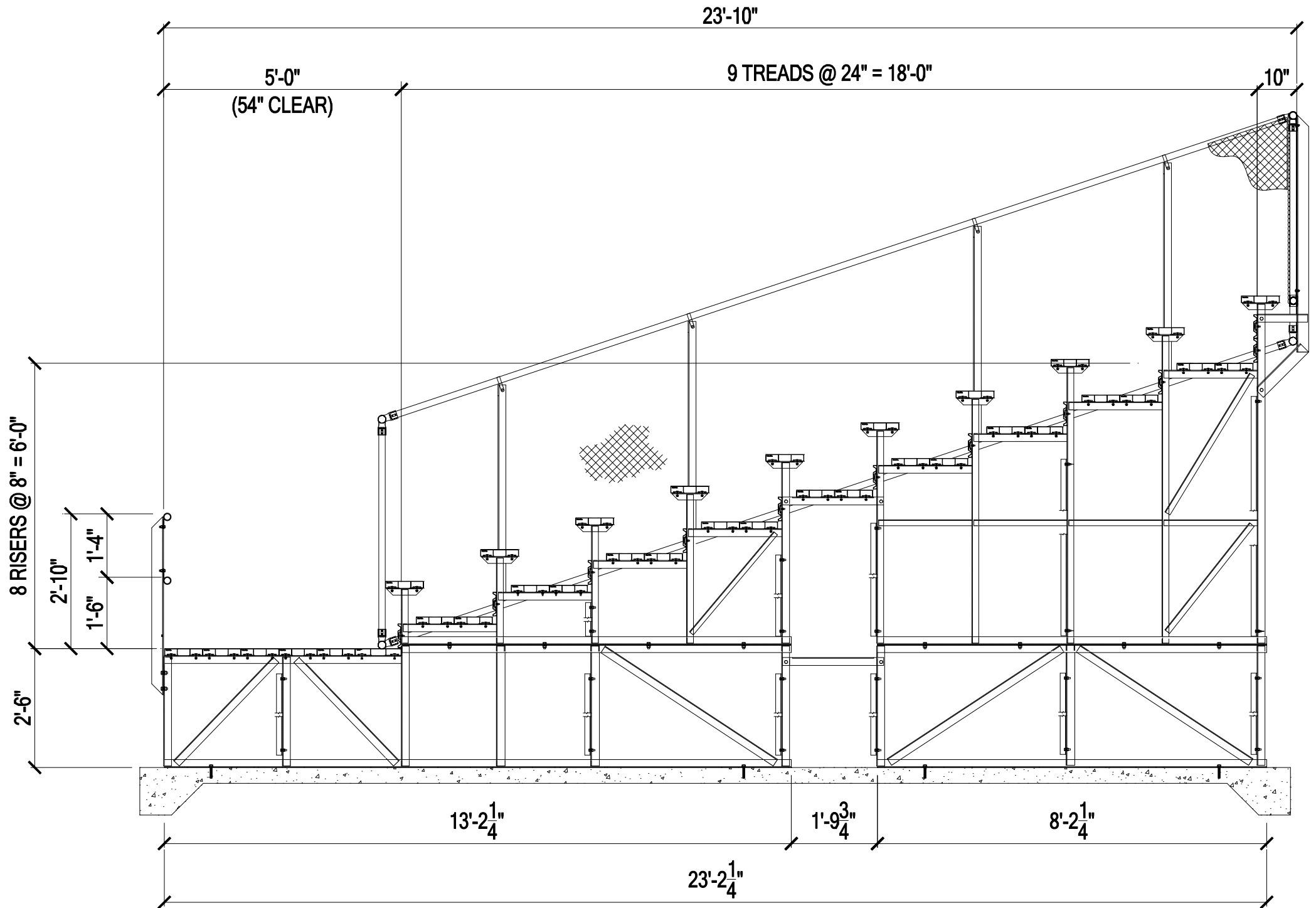
PERMANENT GRANDSTAND - ANGLE FRAME
