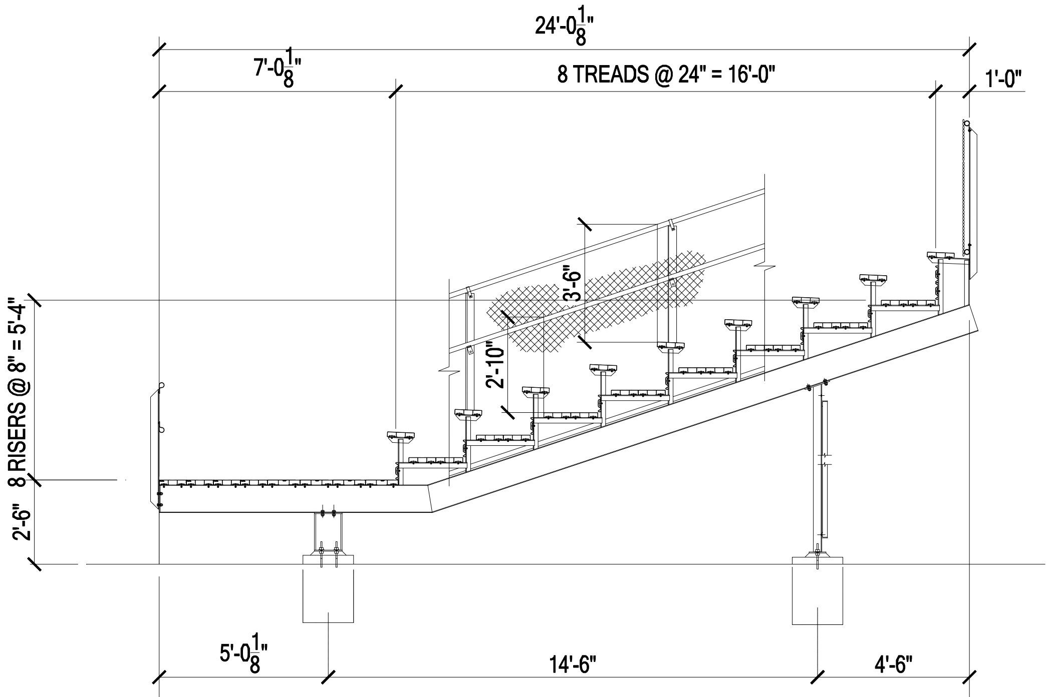
PERMANENT GRANDSTAND - H-FRAME SECTION
