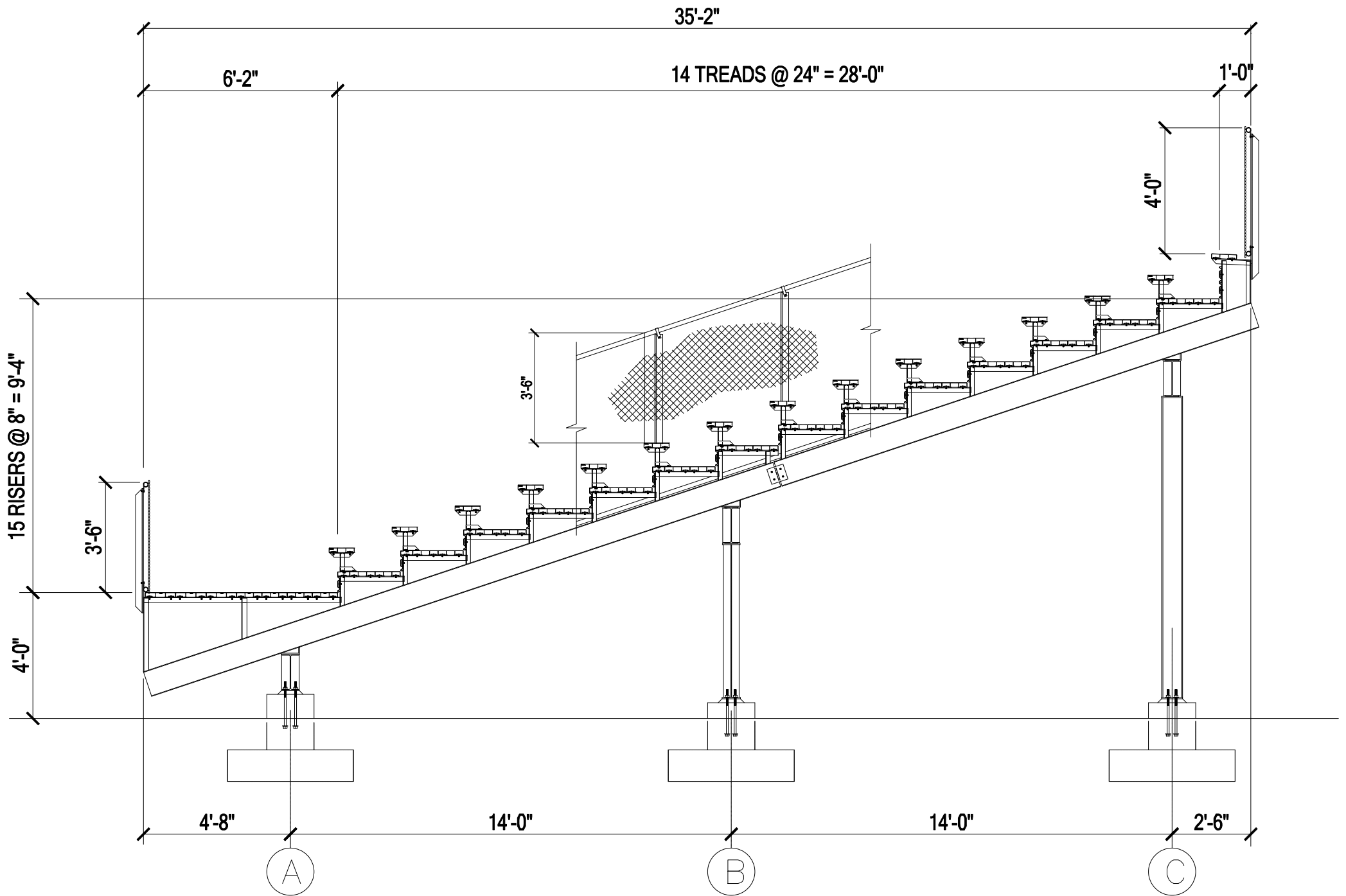
PERMANENT GRANDSTAND - I-BEAM
