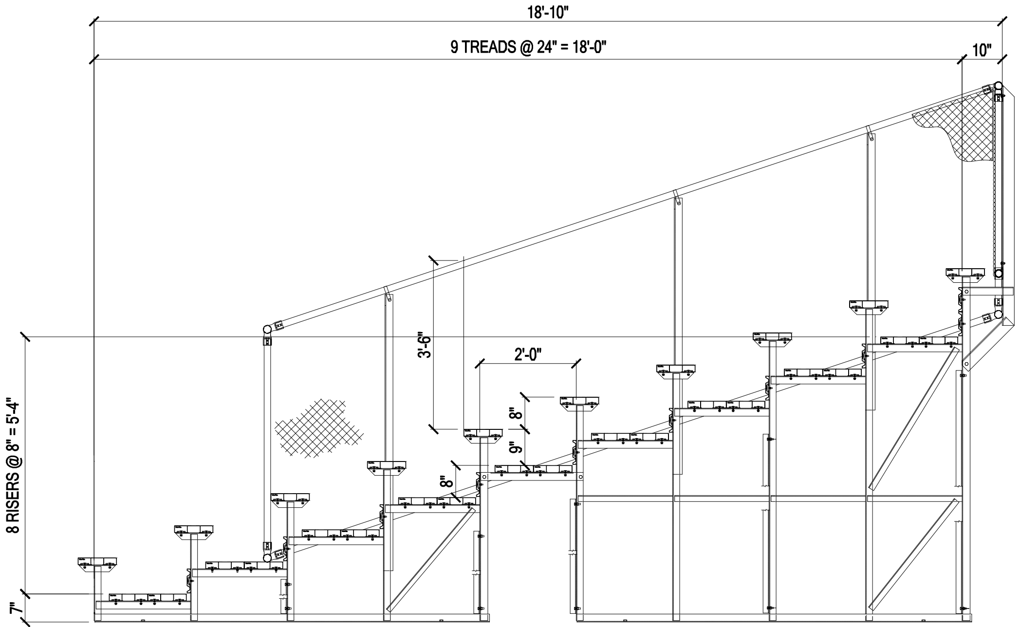
STANDARD SERIES - 10 ROW SECTION
