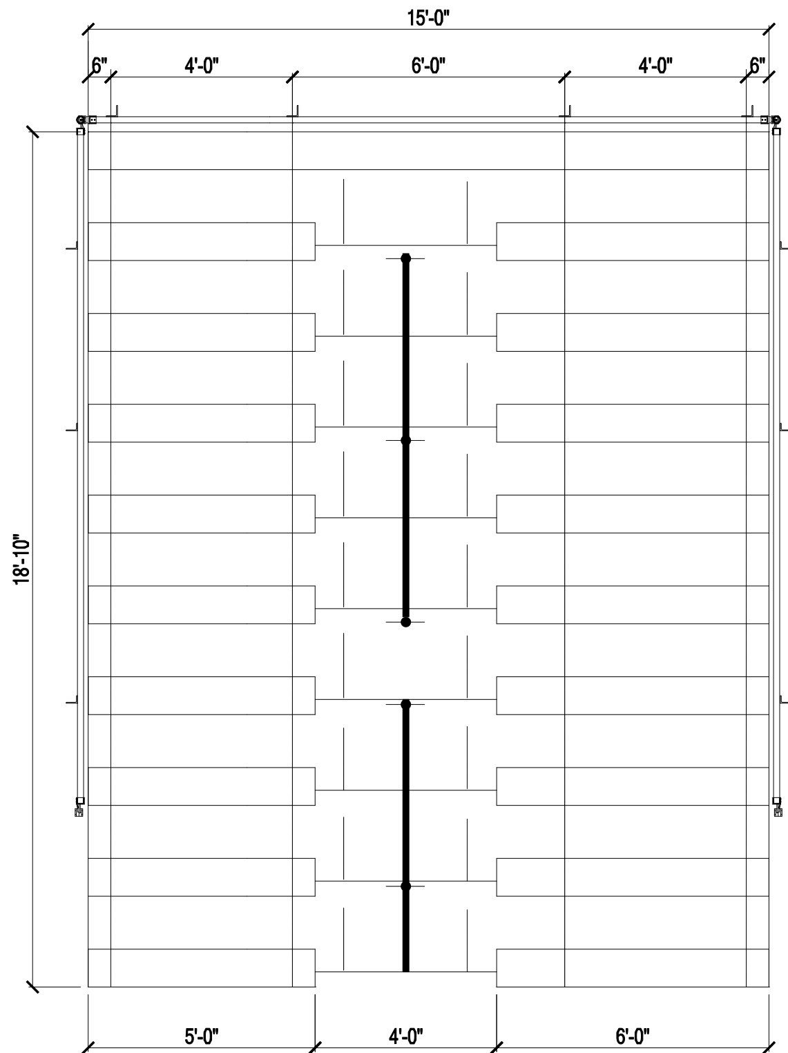
STANDARD SERIES 10 ROW x 15' SEATING PLAN (73 SEATS)
