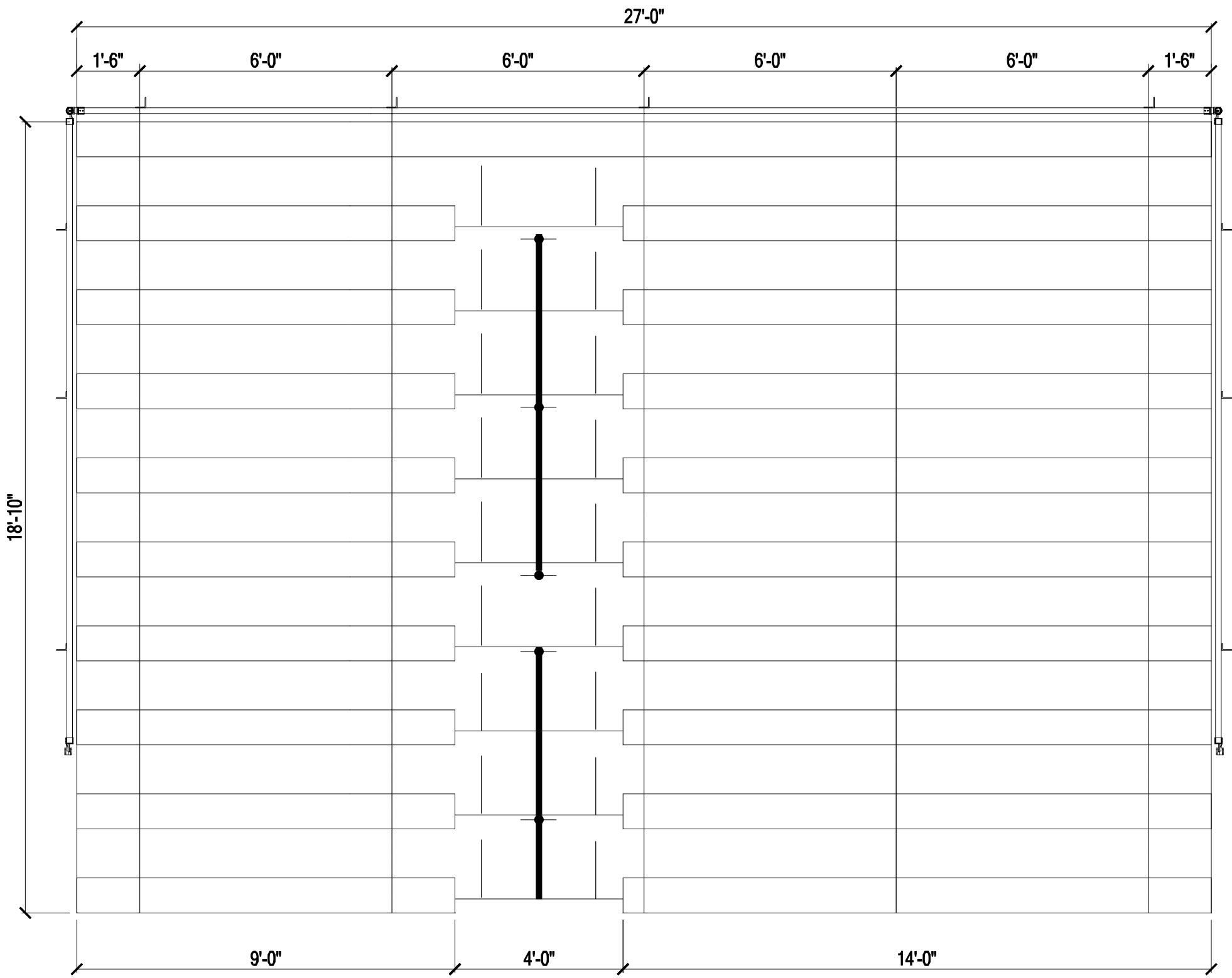
STANDARD SERIES 10 ROW x 27' SEATING PLAN (153 SEATS)
