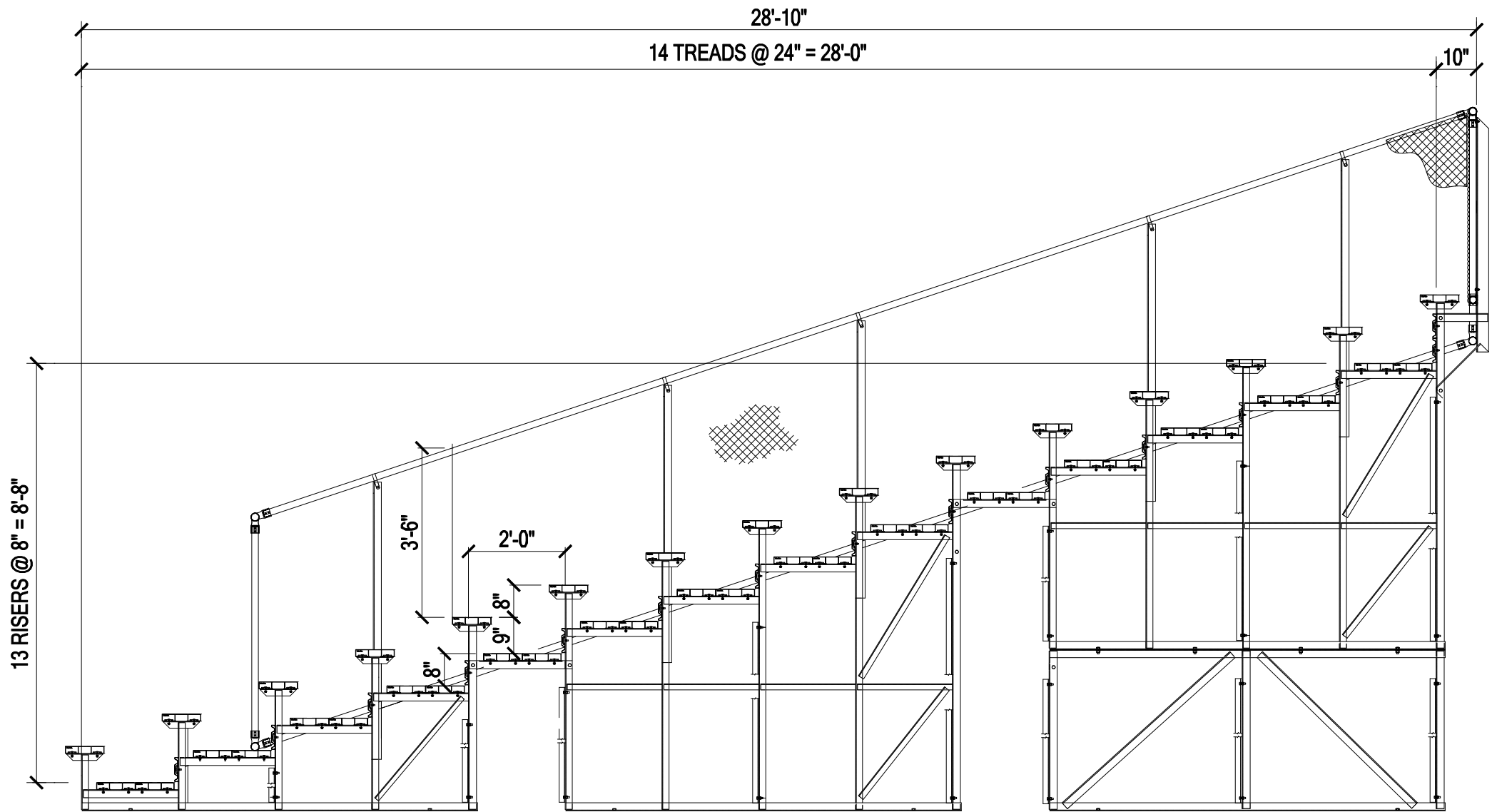
STANDARD SERIES – 15 ROW SECTION
