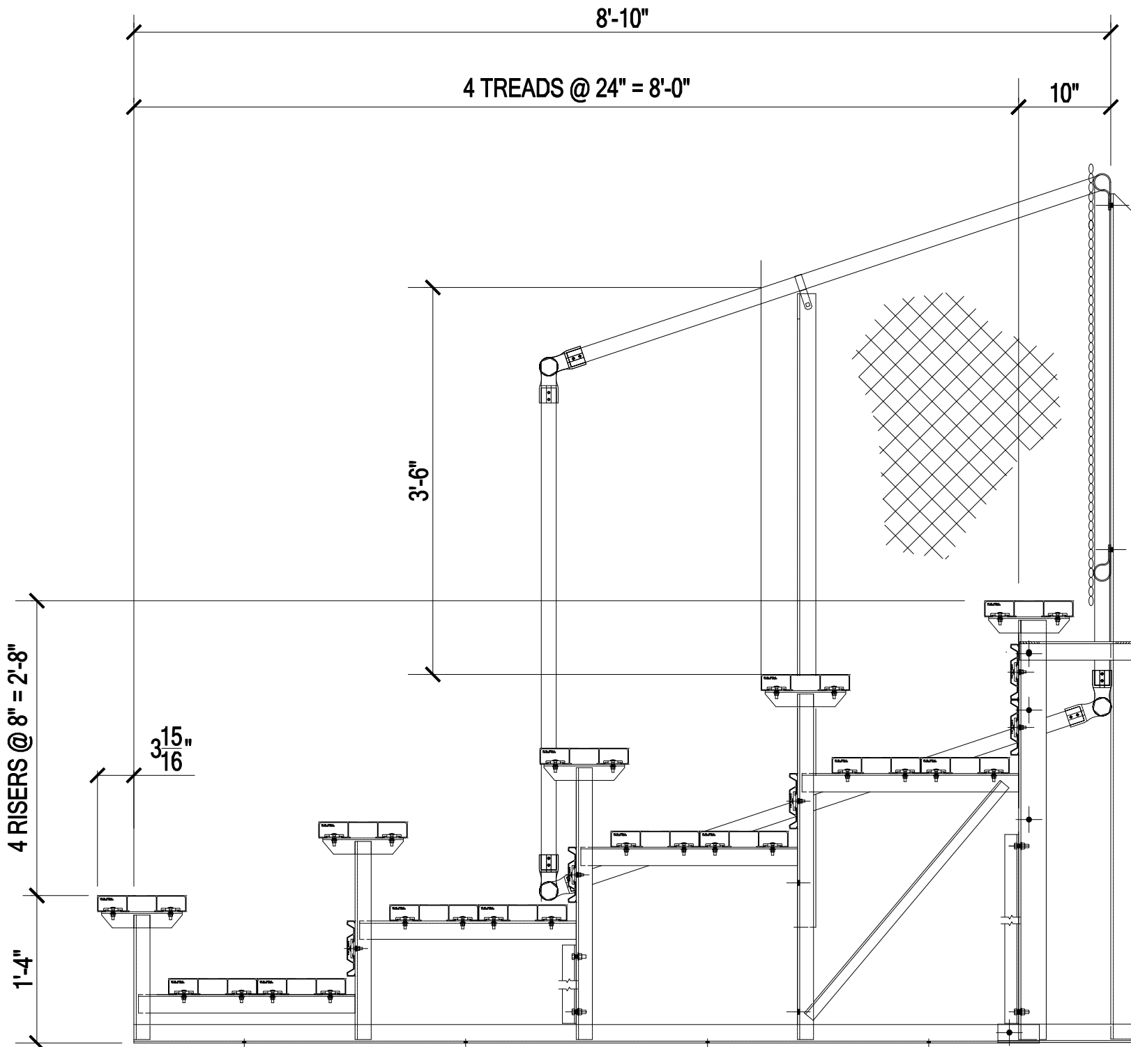
STANDARD SERIES - 5 ROW SECTION
