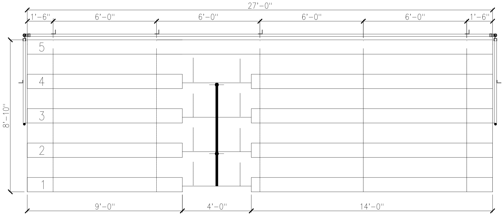
STANDARD SERIES - 5 ROW x 27' SEATING PLAN (78 SEATS)
