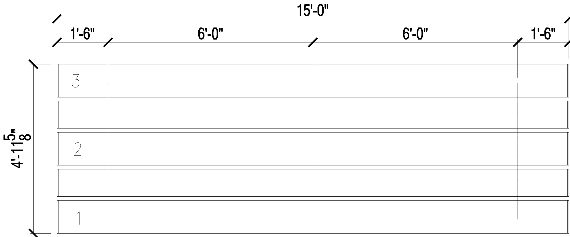
UNIVERSAL SERIES - 3 ROW x 15' SEATING PLAN (30 SEATS)
