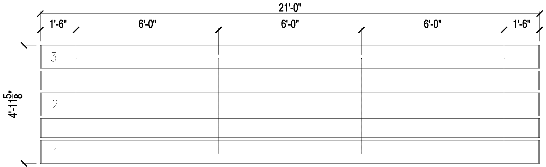
UNIVERSAL SERIES - 3 ROW x 21' SEATING PLAN (42 SEATS)
