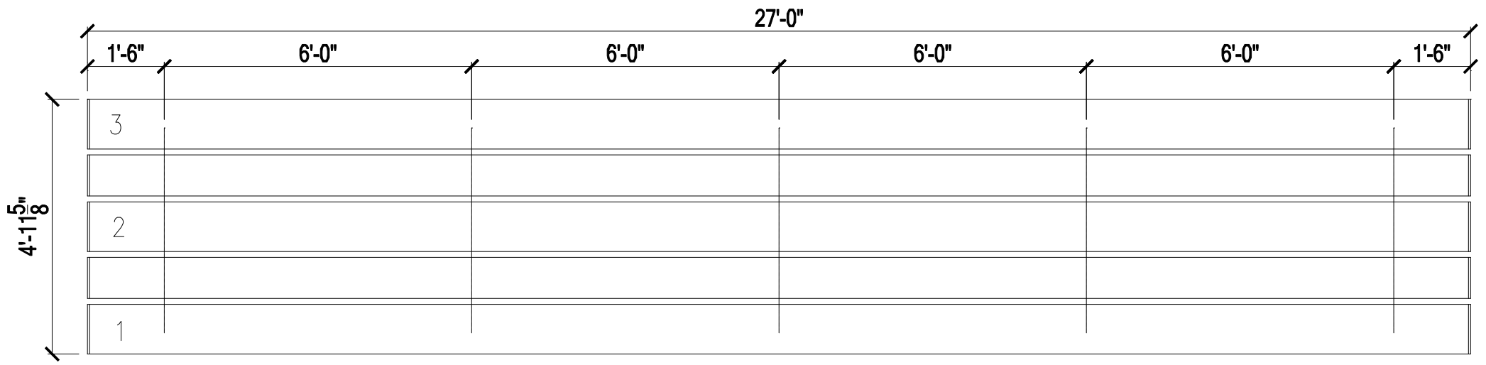
UNIVERSAL SERIES - 3 ROW x 27' SEATING PLAN (54 SEATS)
