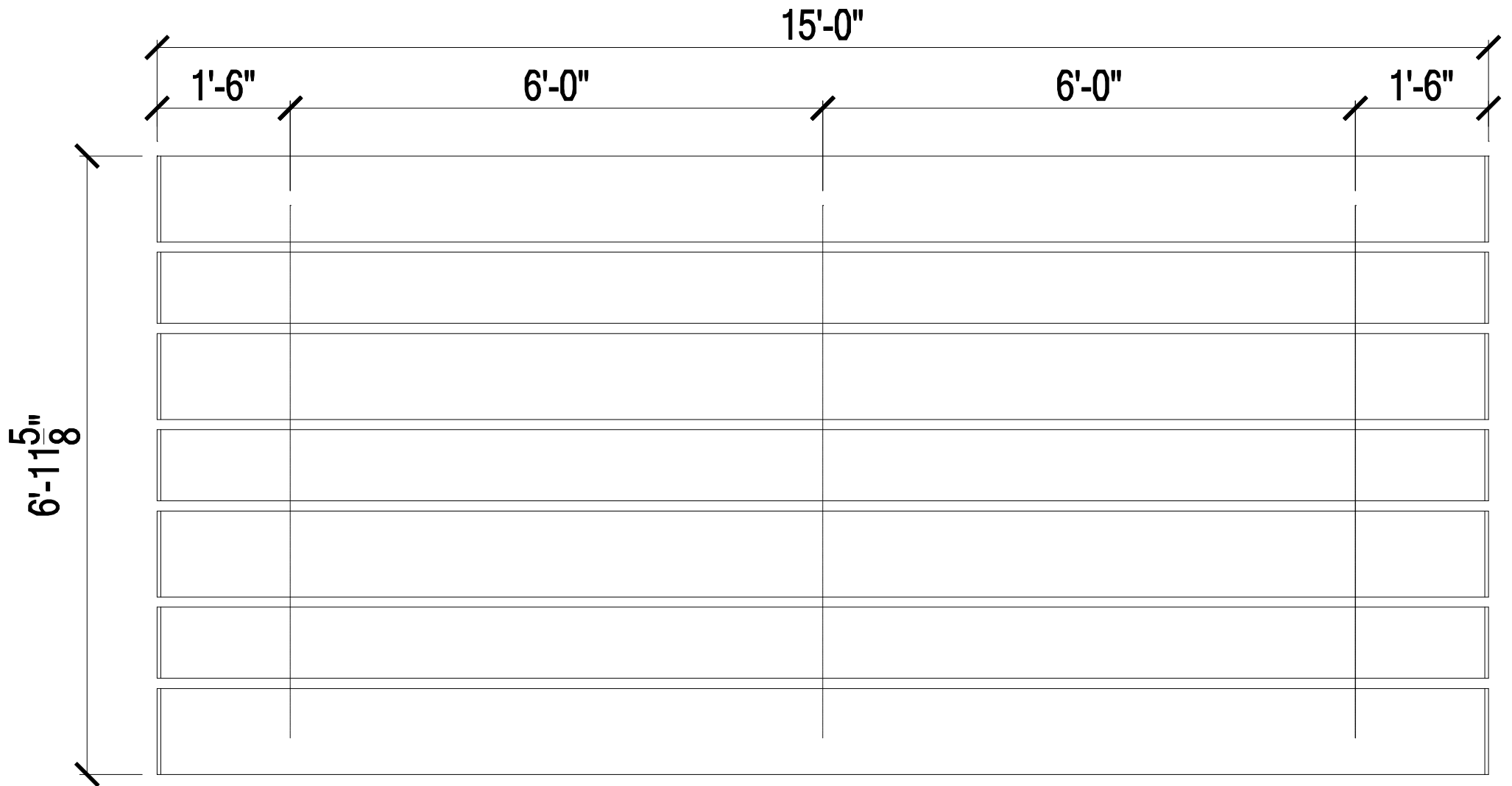
UNIVERSAL SERIES - 4 ROW x 15' SEATING PLAN (40 SEATS)
