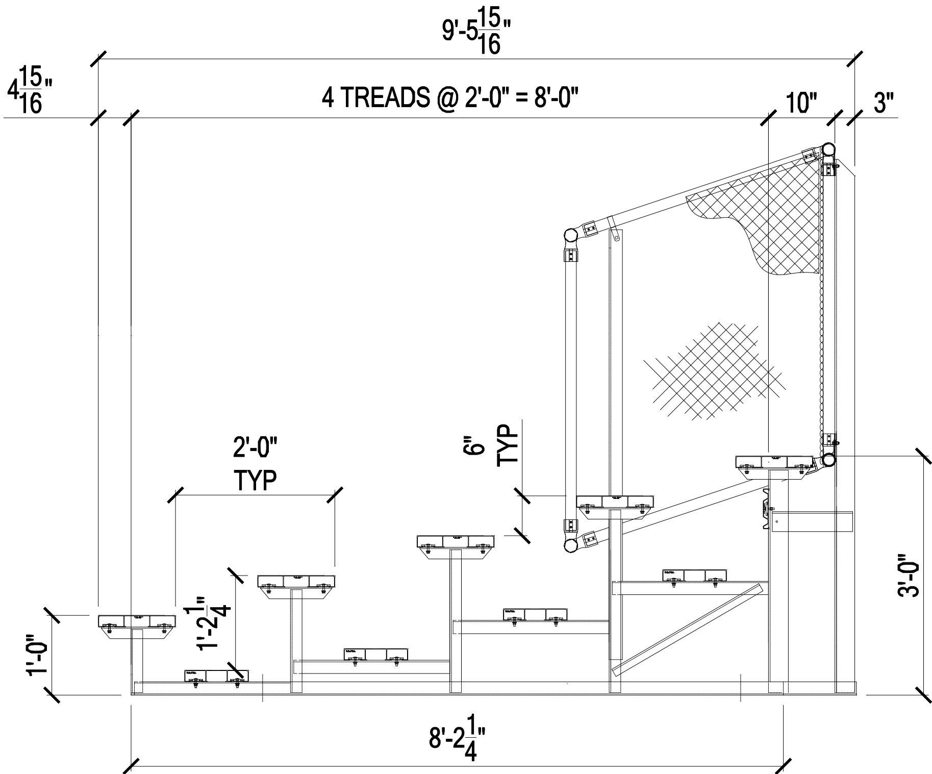
UNIVERSAL SERIES - 5 ROW SECTION
