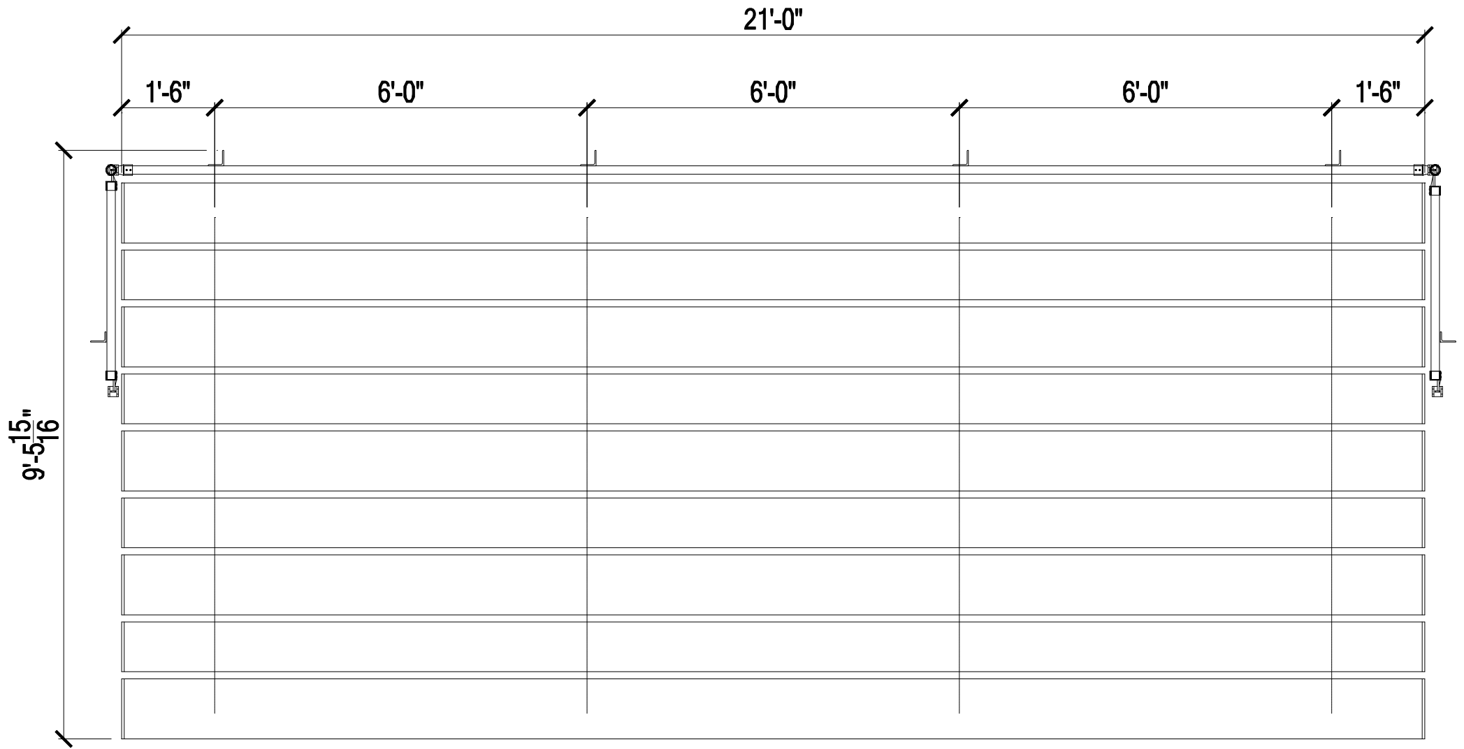
UNIVERSAL SERIES - 5 ROW x 21' SEATING PLAN (70 SEATS)
