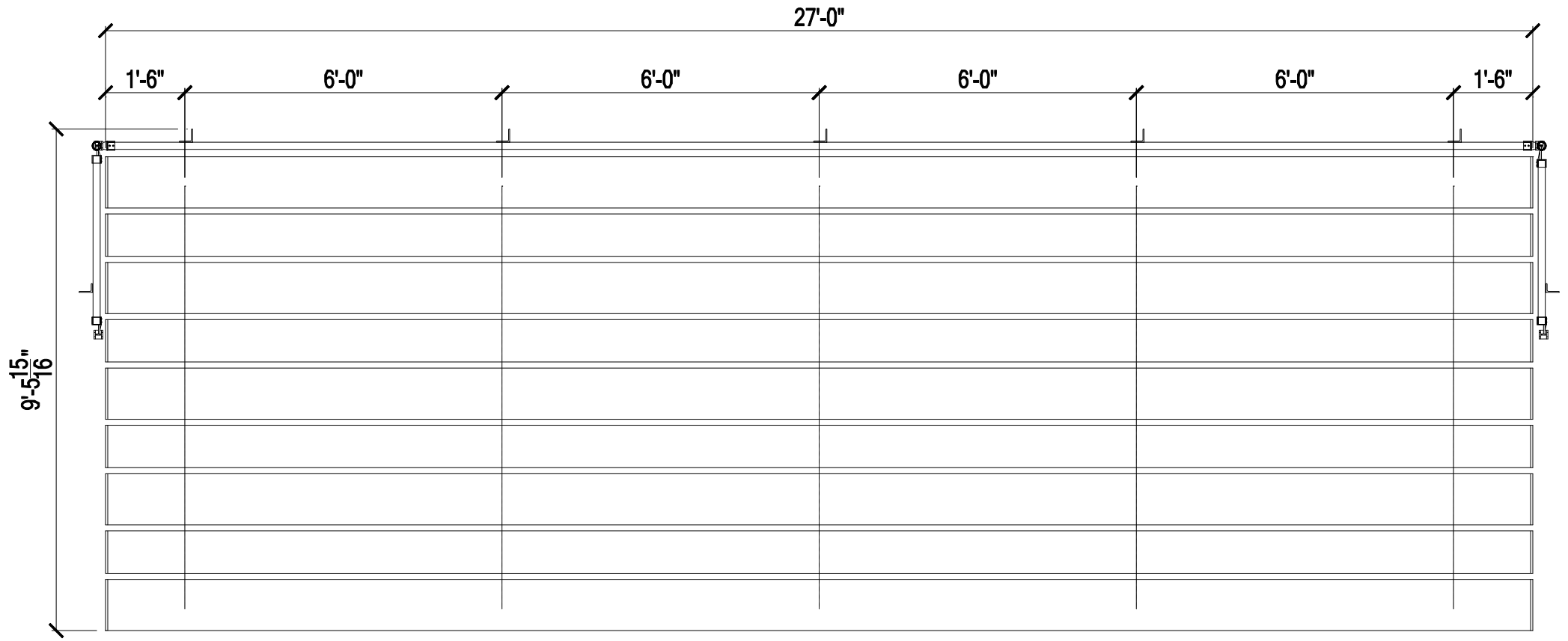
UNIVERSAL SERIES - 5 ROW x 27' SEATING PLAN (90 SEATS)
