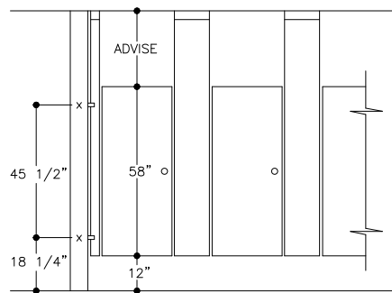
FRONT ELEV
