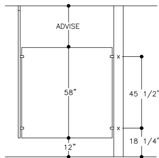
PANEL ELEV
