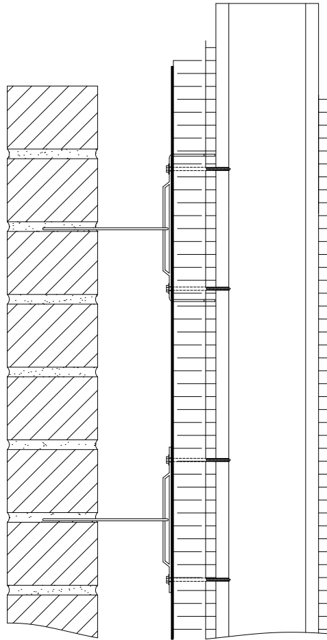
SECTION VIEW
