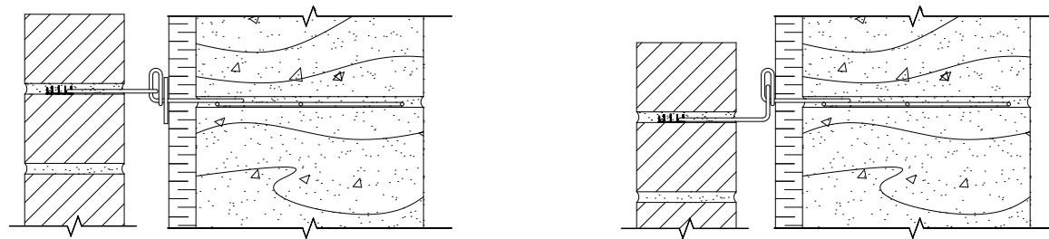
SECTION VIEW
