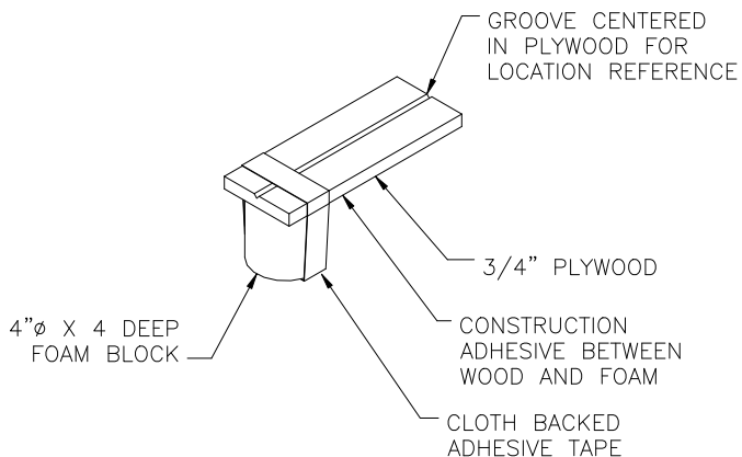
— FOAM BLOCK OUT DETAIL SCALE: 3
