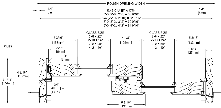
French Horizontal 2-Wide Section View
