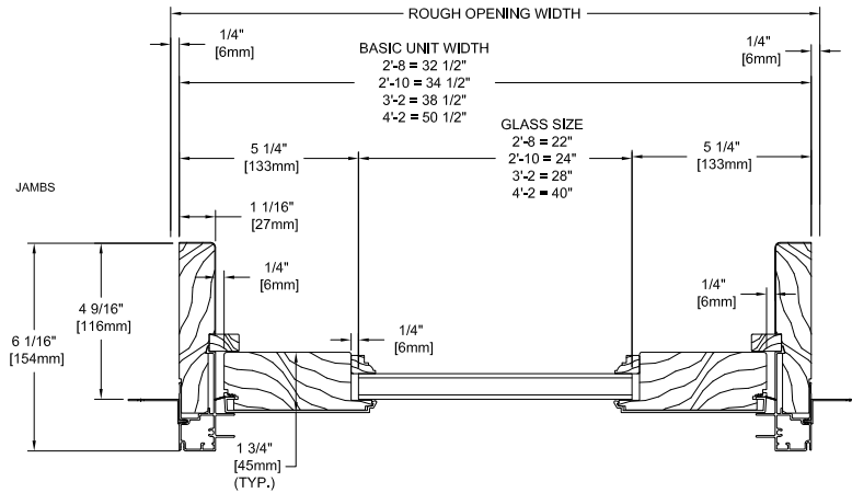
French Horizontal Stationary Section View
