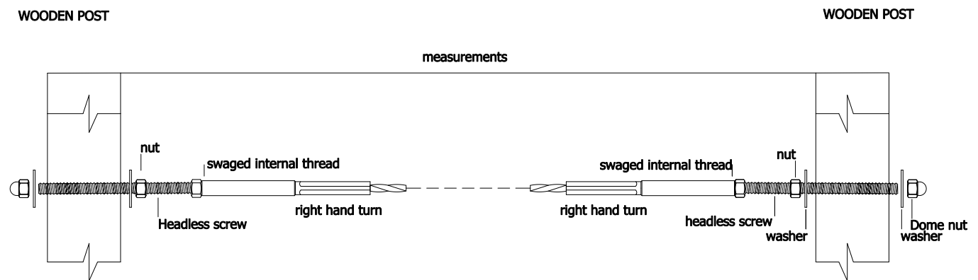
ASSEMBLY 3
