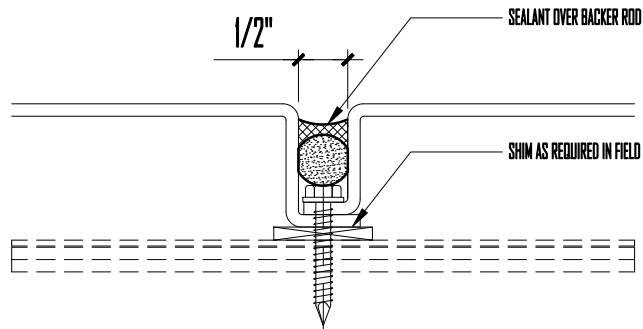
2. PARAPET JOINT
