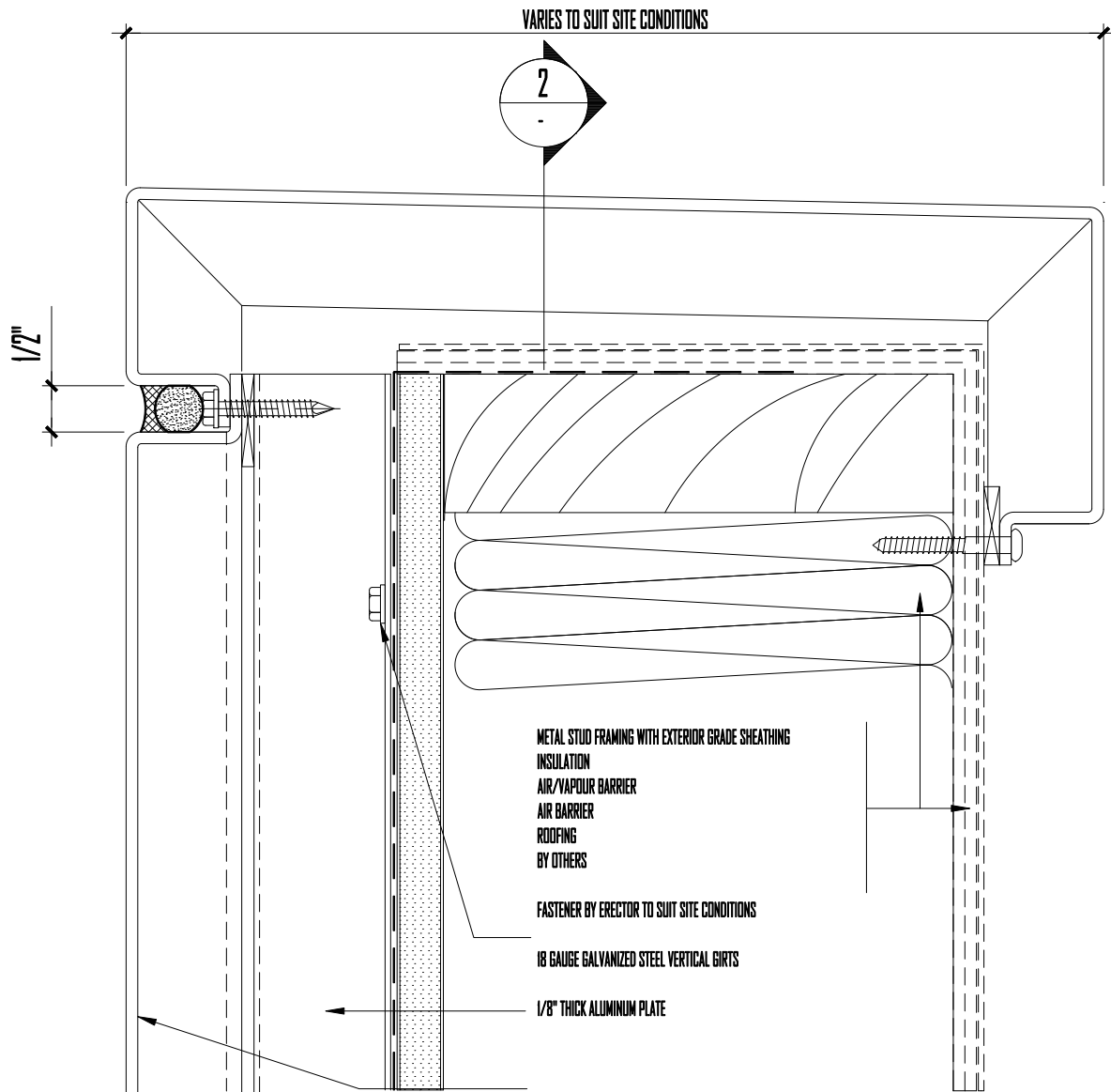
1. PARAPET DETAIL
