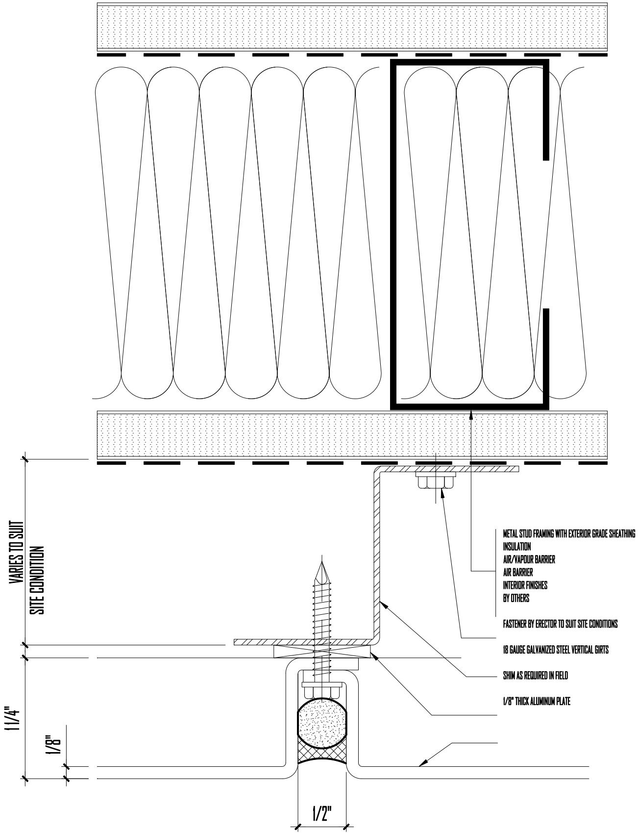
4. VERTICAL JOINT
