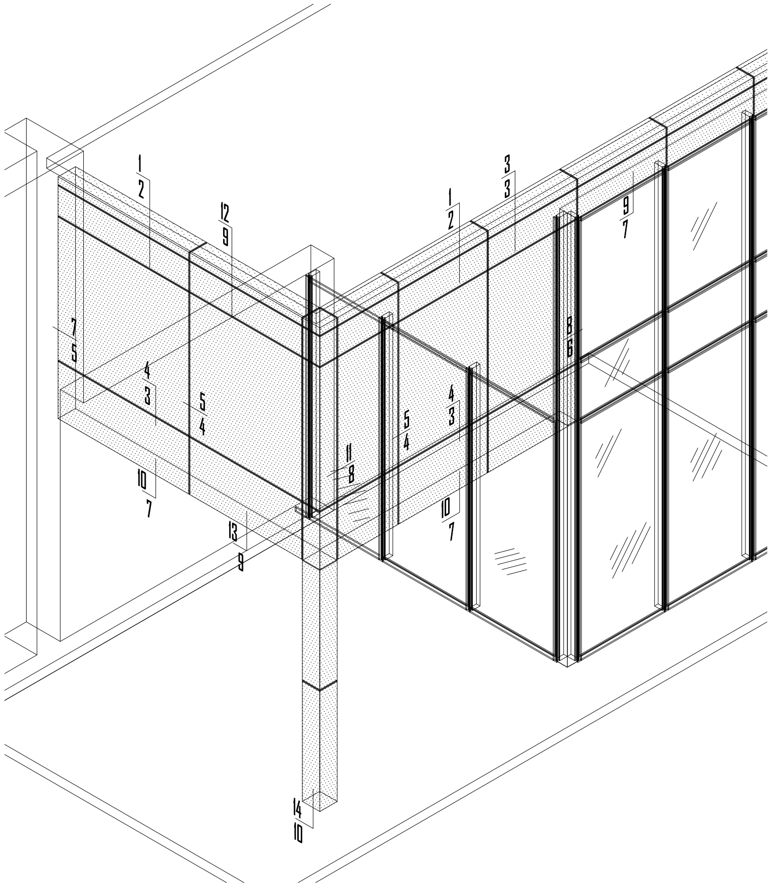
PARTIAL ELEVATION
