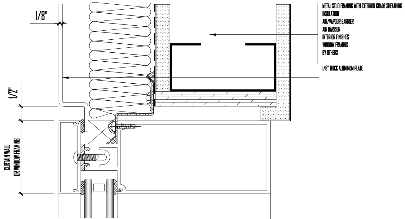
9. WINDOW HEAD
