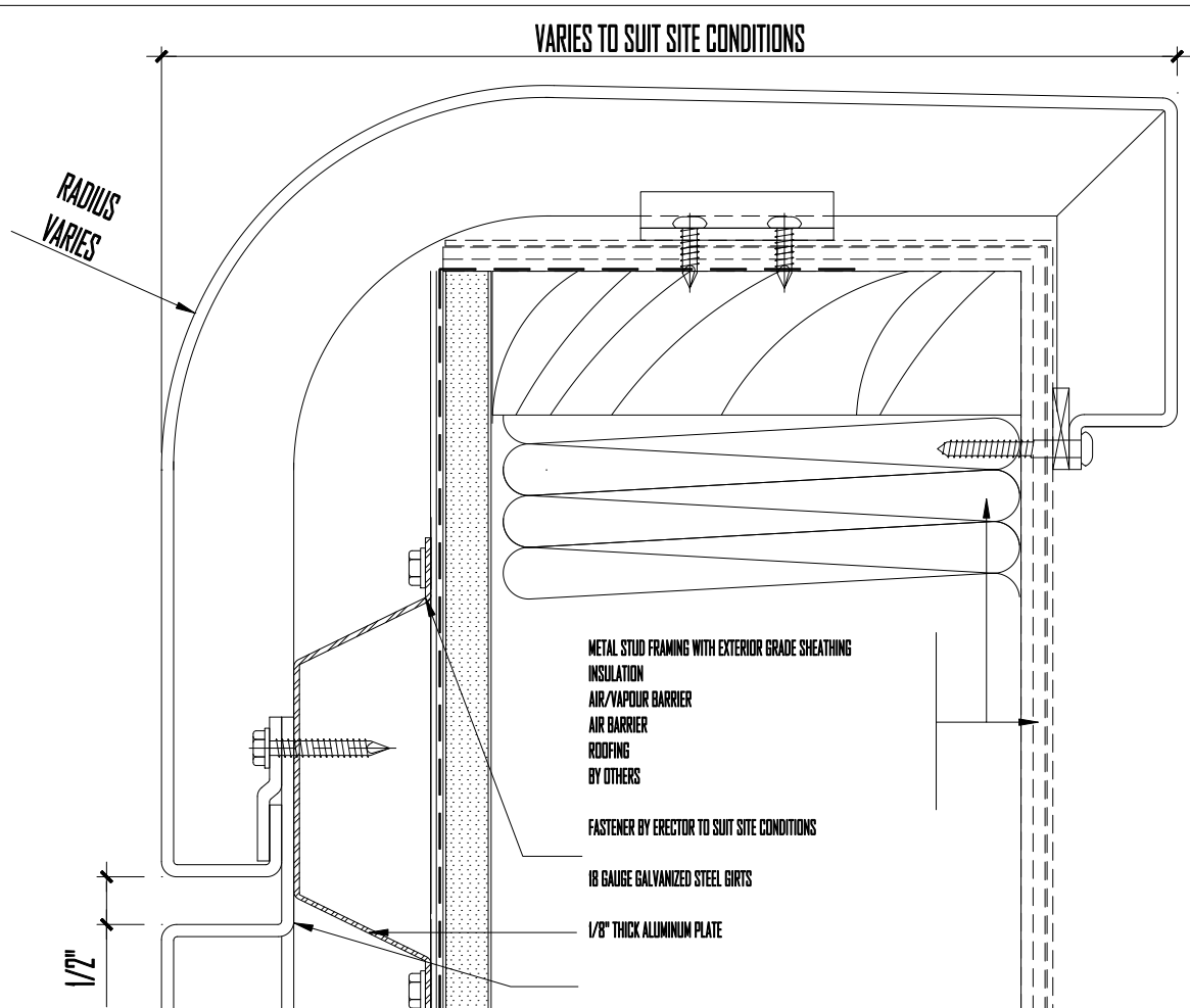
12. PARAPET DETAIL
