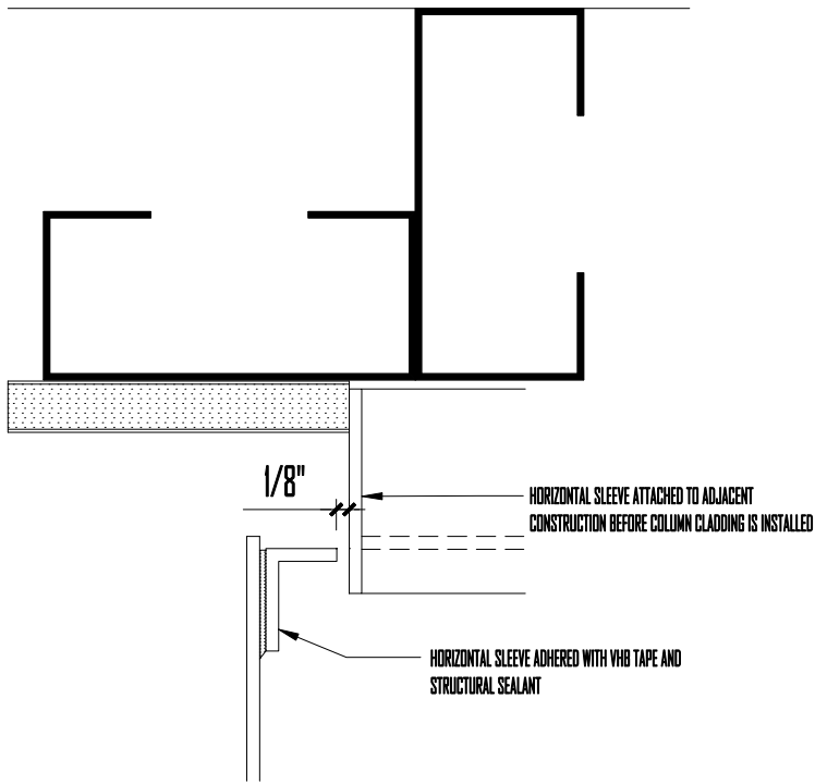
9. TOP OF COVER
