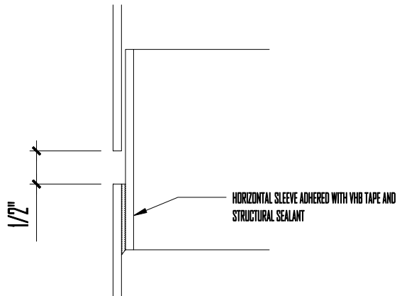
10. INTERMEDIATE JOINT
