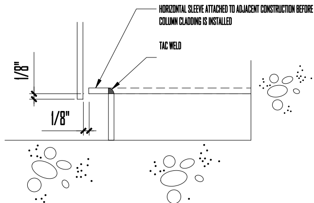
11. BOTTOM OF COVER
