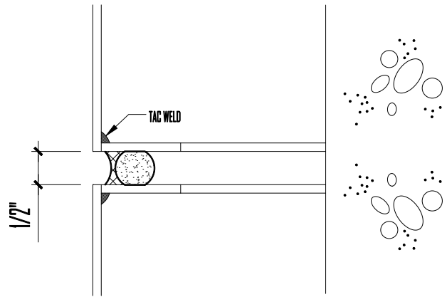
10A. ALTERNATE JOINT
