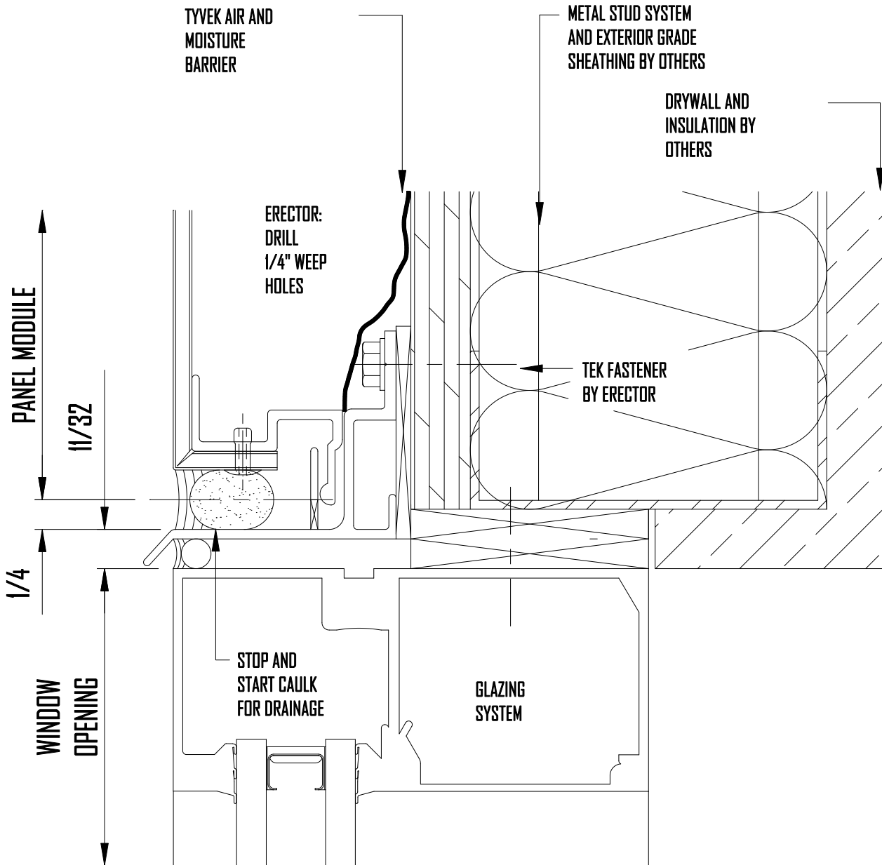
04 GLAZING SYSTEM HEAD
