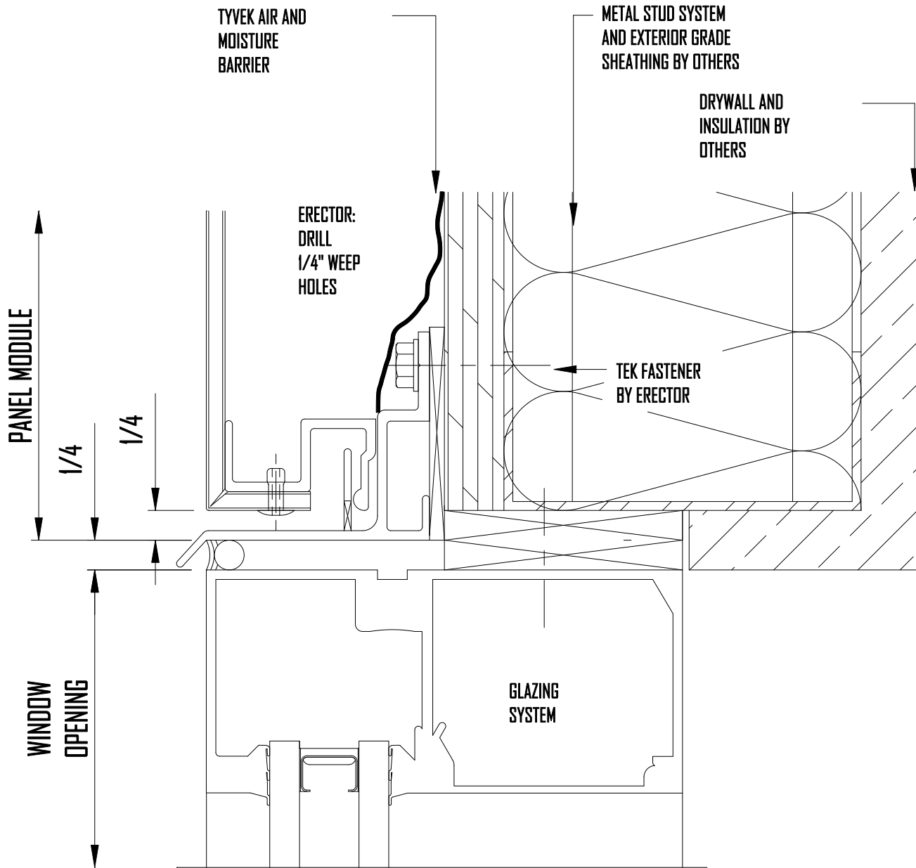
D4A GLAZING SYSTEM HEAD
