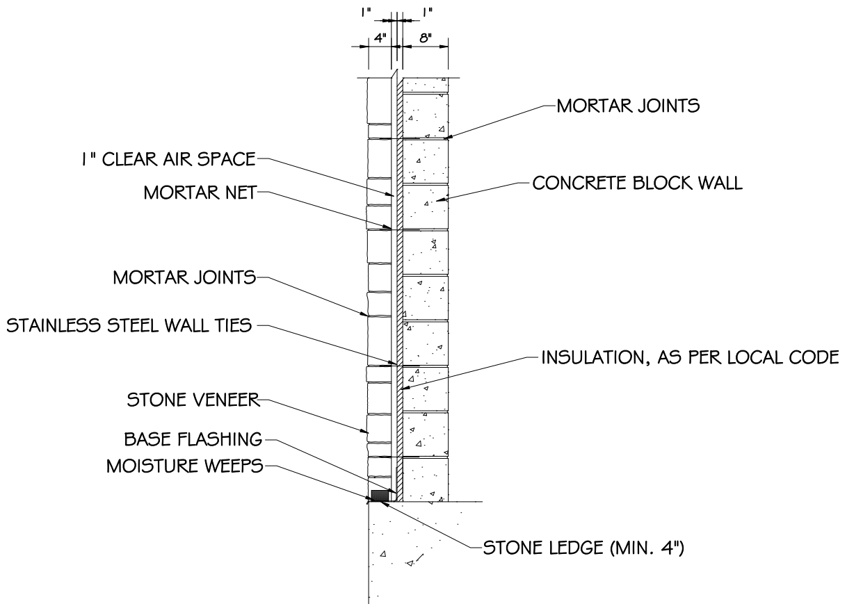
TYPICAL SECTION FOR CONCRETE BLOCK WALL
