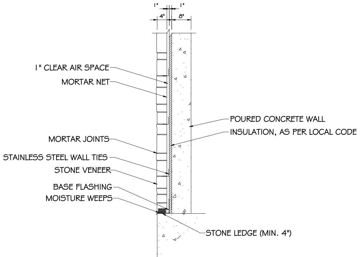
TYPICAL SECTION FOR Poured CONCRETE WALL
