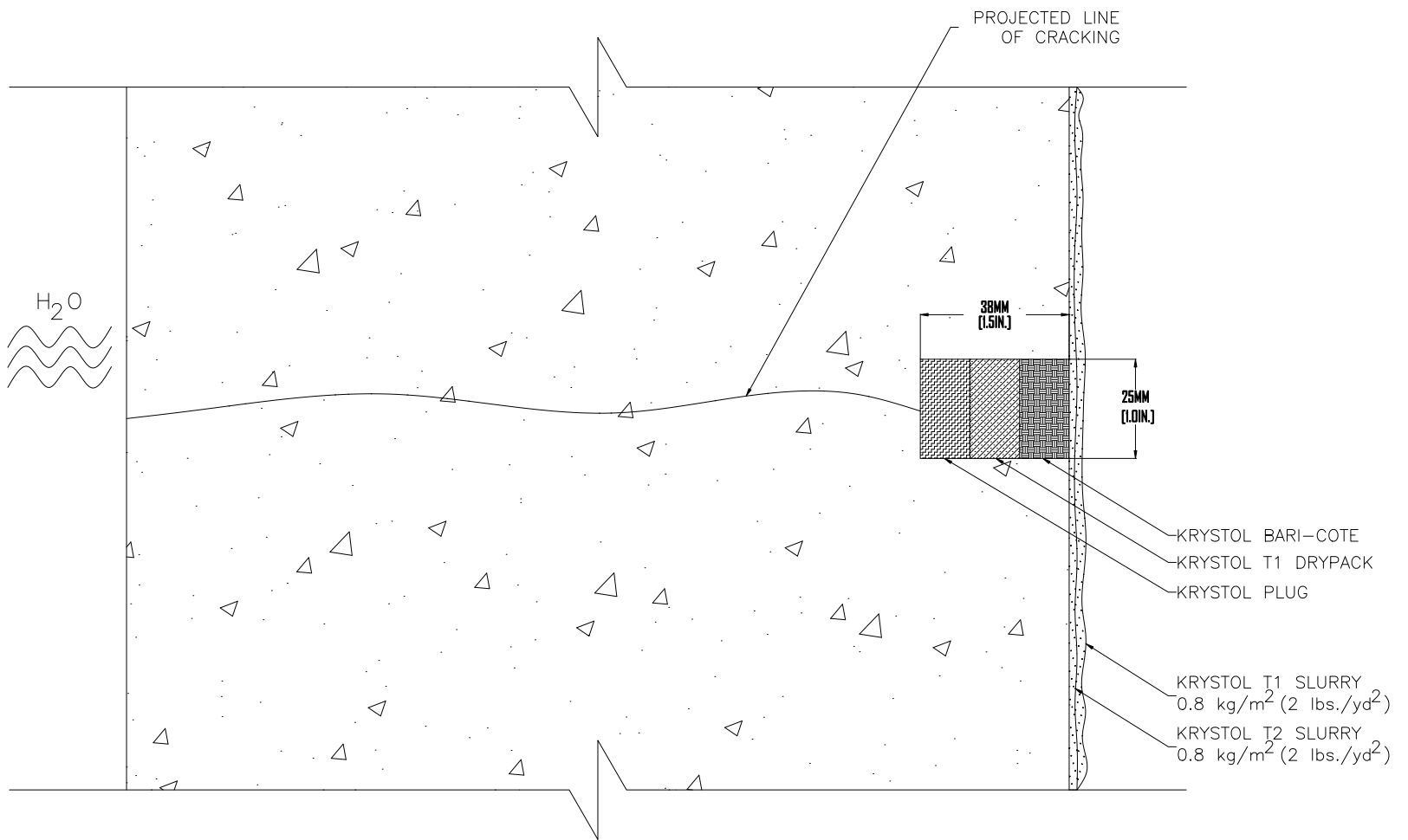
NEGATIVE SIDE CRACK REPAIR (CROSS SECTION)
