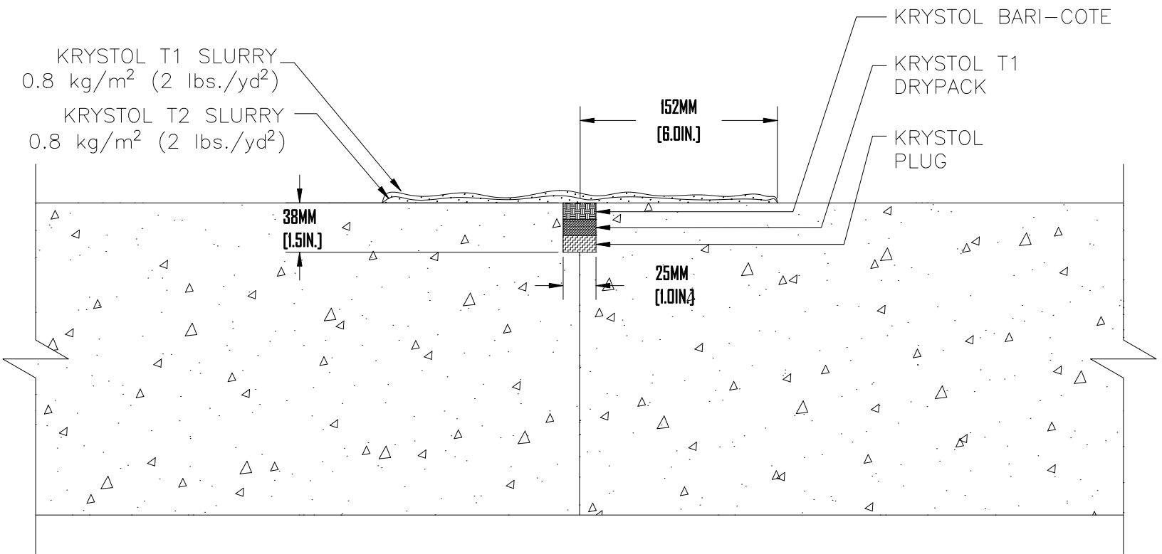
CRACK OR JOINT REPAIR — SLAB TO SLAB
