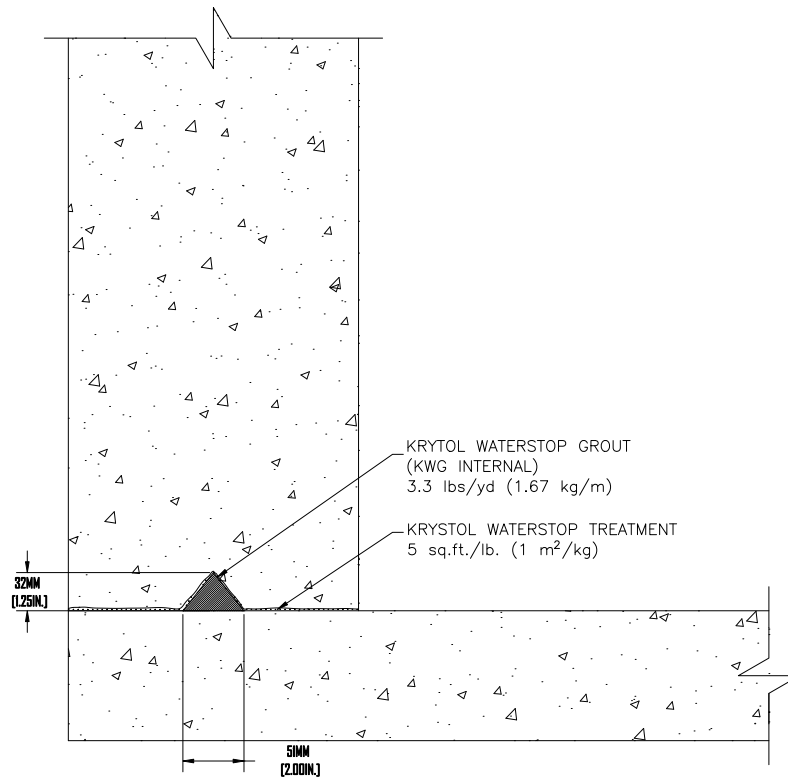
NEW CONSTRUCTION – WALL TO SLAB (WALL ON TOP OF SLAB)
