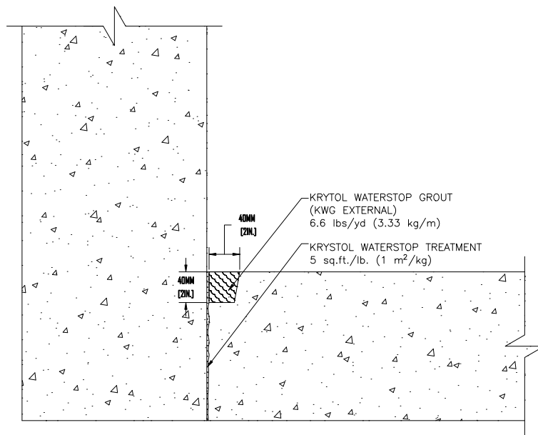
NEW CONSTRUCTION – WALL TO SLAB (WALL INBOARD OF SLAB)
