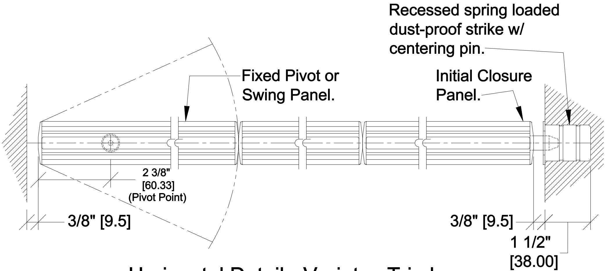
Horizontal Detail - Variotec Trimless
