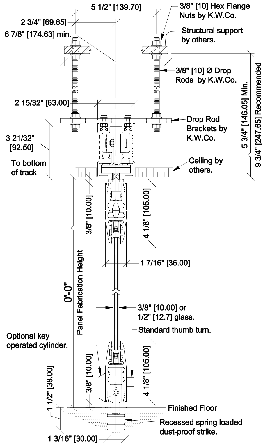
Vertical Detail Variotec Trimless
