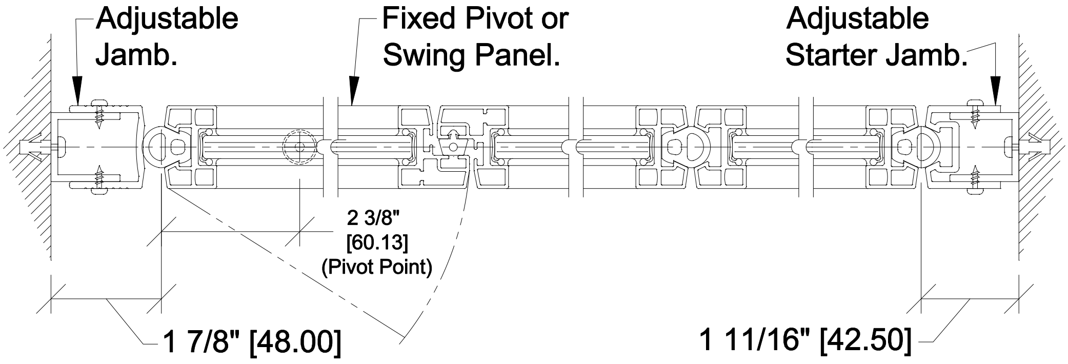
Horizontal Detail - Variotec Trimmed
