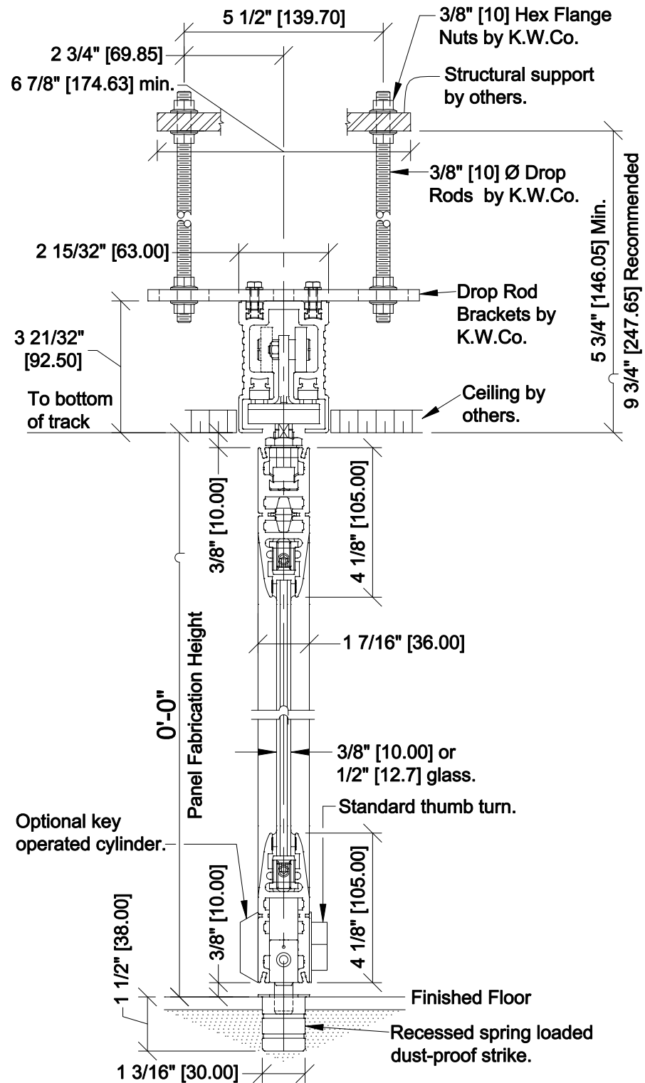
Vertical Detail Variotec Trimmed
